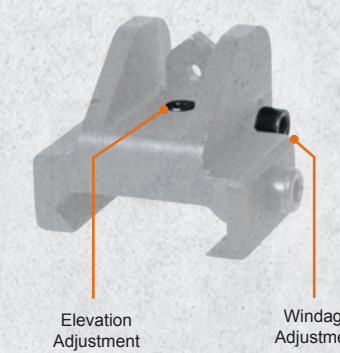
MNT-722 Clamp-on Front Sight With Elevation Adjustable Front Sight Post
